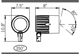
Floodlight Detail
