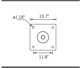
Mounting Detail
